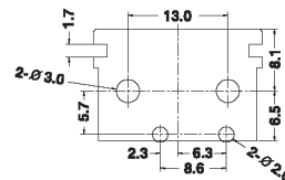
Suggested panel hole size
